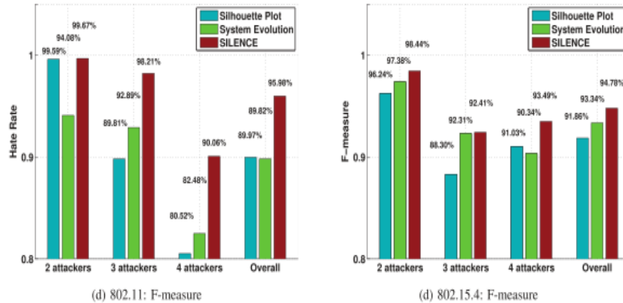
Fig.4 Hit Rate and F-Measure Comparison Of SILENCE To Strategies Exploitation Cluster Analysis Alone Like Silhouette And System Evolution.
