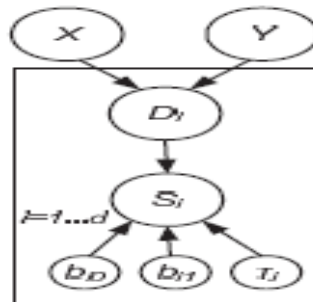
Fig 3. Bayesian Network in Proposed Model
