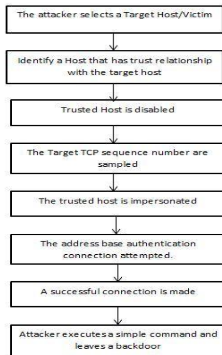
Fig.1 Procedure in spotting attack
